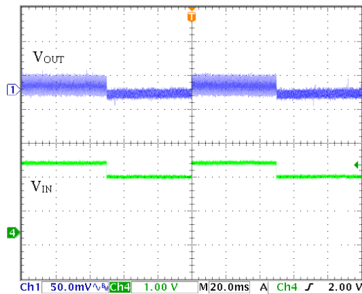
Fig 34. HT7727S Line Transient Response (L= 10μH, C IN = C OUT = 10μF, V IN = 1.62V)
