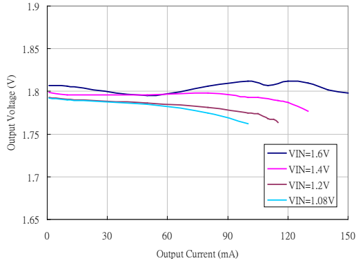
Fig 45. HT7718S Output Voltage vs. Output Current
