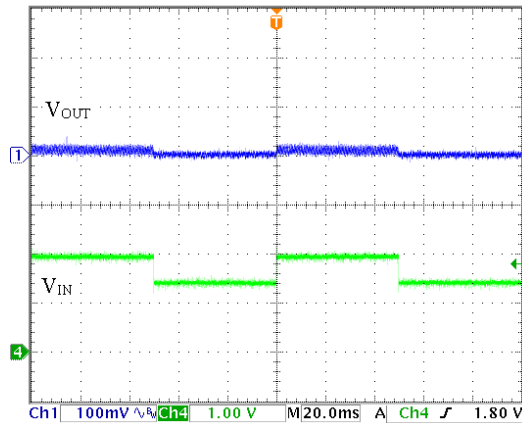
Fig 22. HT7733S Line Transient Response (L=10µH, C IN =C OUT =10µF, V IN =1.98V)
