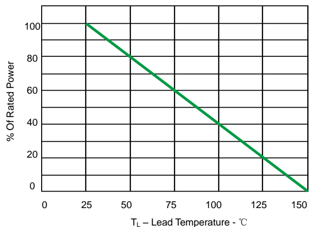
Fig 2.Power Derating Curve
