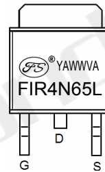
Marking Diagram
