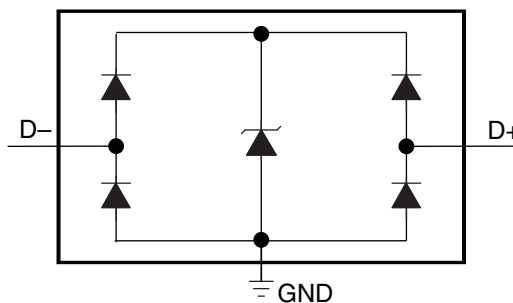
TPD2EUSB30/A Circuit
