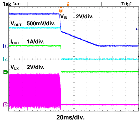
Figure 11. Power Off through VIN Waveform
