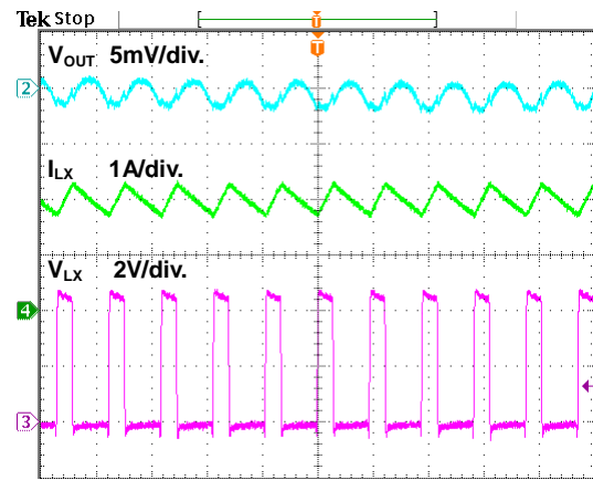
Figure 17. Steady State Waveform
