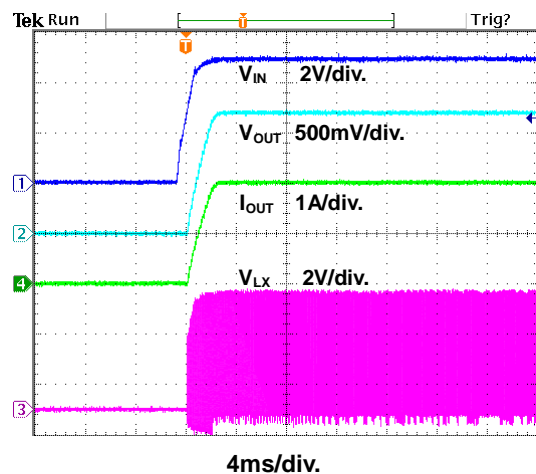
Figure 9. Power On through VIN Waveform
