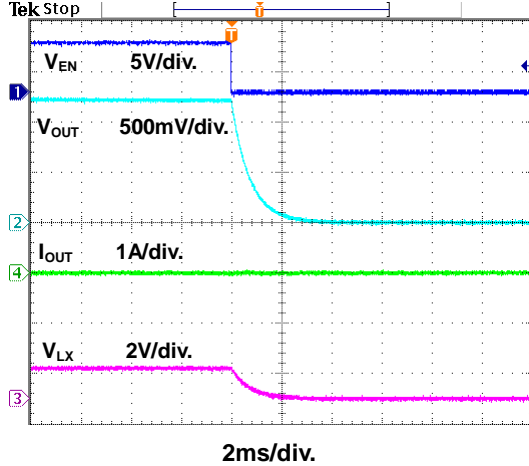
Figure 14. Power Off through EN Waveform
