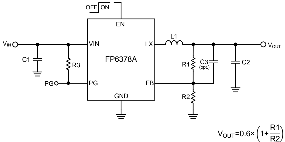
Figure 2. Schematic Diagram
