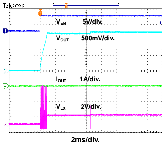
Figure 12. Power On through EN Waveform
