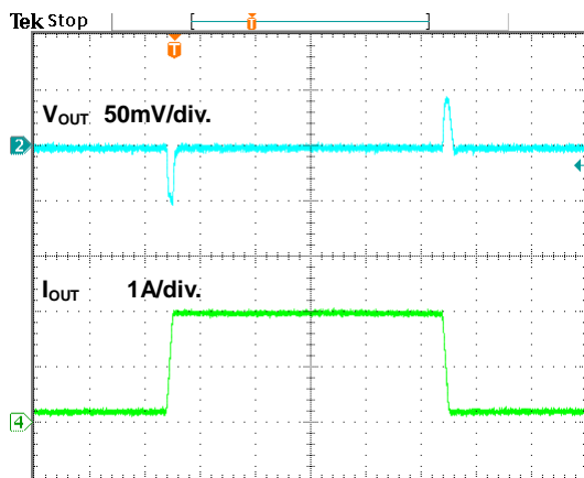
Figure 18. Load Transient Waveform
