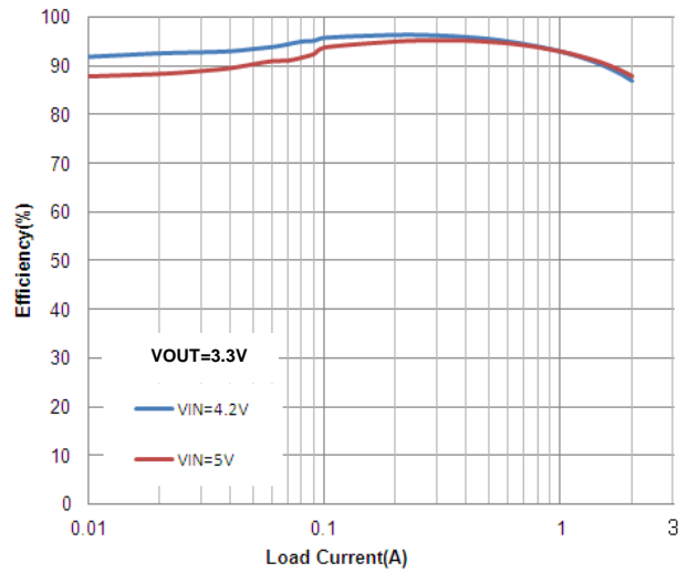
Figure 5. Efficiency vs. Load Current
