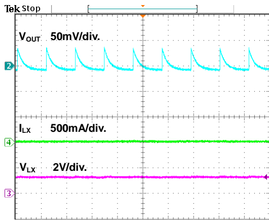
Figure 16. Steady State Waveform
