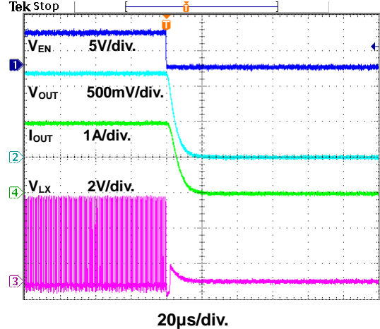
Figure 15. Power Off through EN Waveform
