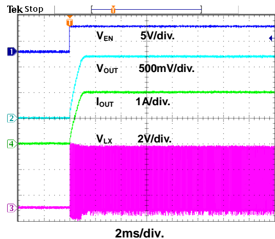
Figure 13. Power On through EN Waveform
