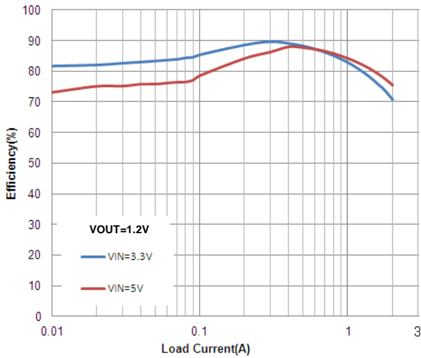
Figure 4. Efficiency vs. Load Current
