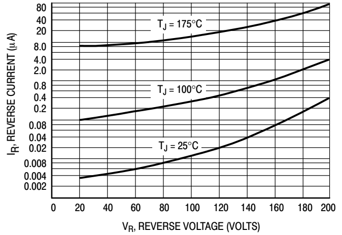
Figure 2. Typical Reverse Current* *The curves shown are typical for the highest voltage device in the voltage grouping. Typical reverse current for lower voltage selections can be estimated from these same curves if applied V_R is sufficiently below rated V_R .
