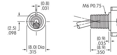
S4 6mm/.350" (8.9mm) Threaded with Keyway
