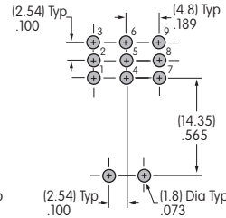
Three Pole
