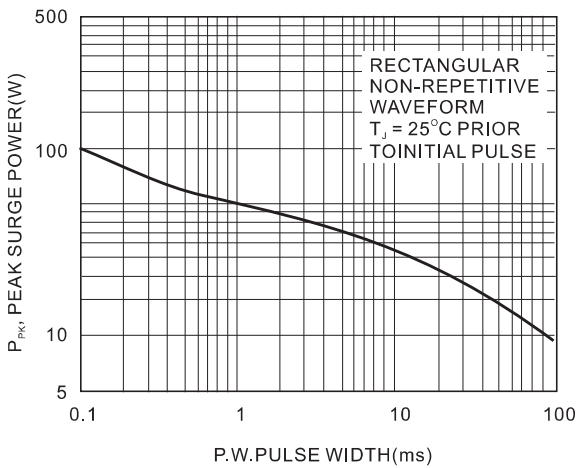
FIG. 2-MAXIMUM SURGE POWER
