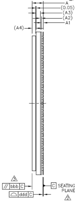
Fig. 2-3 RK3288 FCBGA636LD Package Side View
