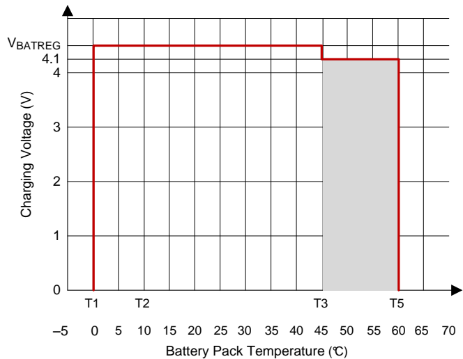
Figure 12. JEITA Profile: Charging Voltage
