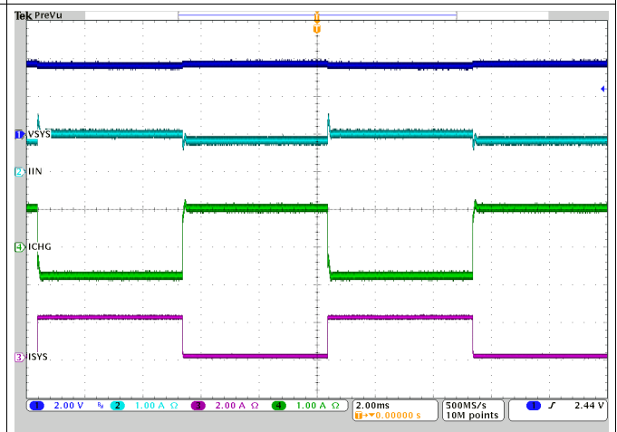
Figure 28. OTG Switching
