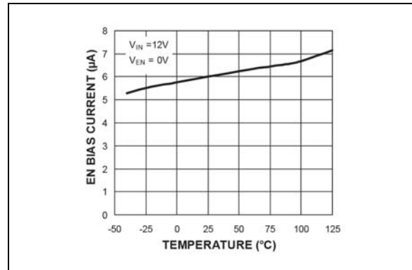
FIGURE 2-54: EN Bias Current vs. Temperature.
