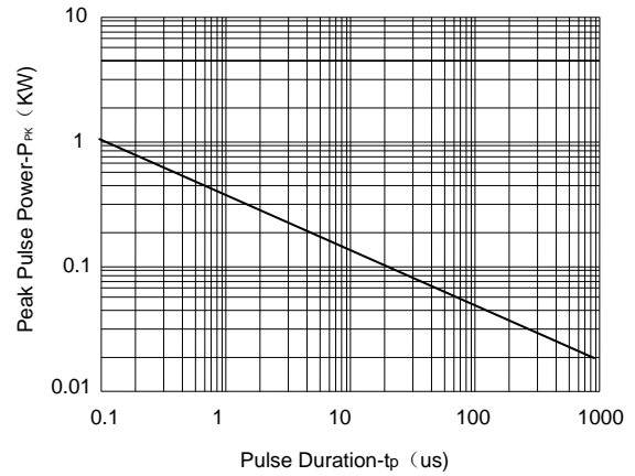
Non-Repitative Peak Pulse Power vs. Pulse Time
