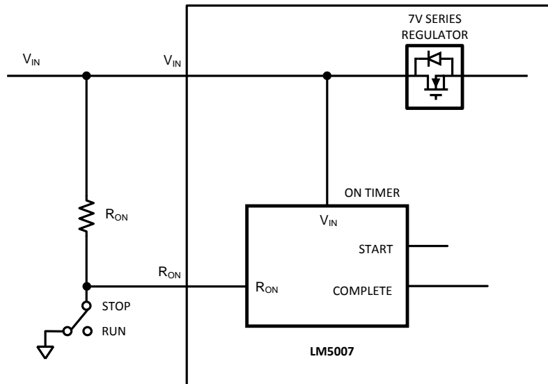
Figure 6. Shutdown Implementation
