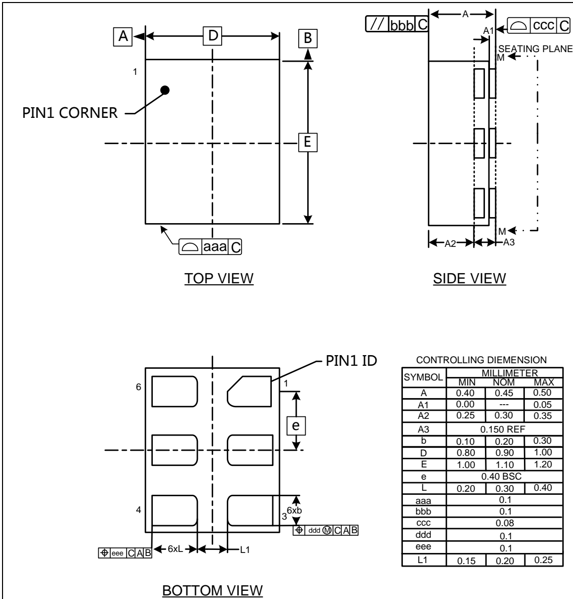
Figure 32. Package Outline
