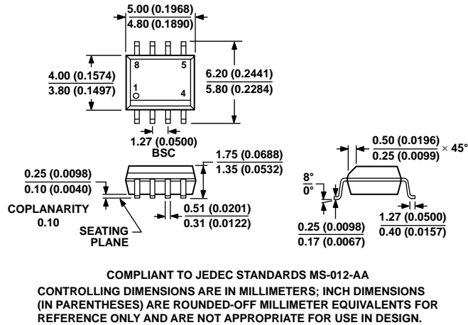
Figure 101. 8-Lead Standard Small Outline Package [SOIC_N] Narrow Body (R-8) Dimensions shown in millimeters and (inches)
