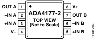
Figure 5. ADA4177-2 8-Lead MSOP Pin Configuration
