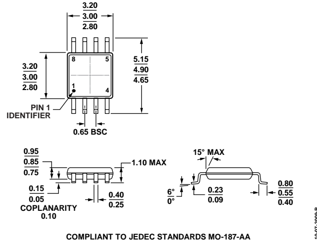
Figure 100. 8-Lead Mini Small Outline Package [MSOP] (RM-8) Dimensions shown in millimeters
