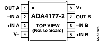
Figure 6. ADA4177-2 8-Lead SOIC Pin Configuration
