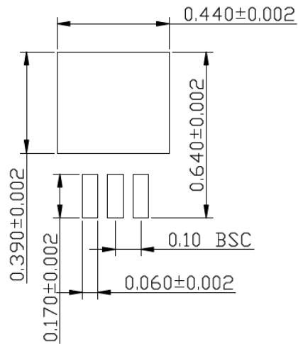
RECOMMENDED LAND PATTERN (UNIT: INCH)
