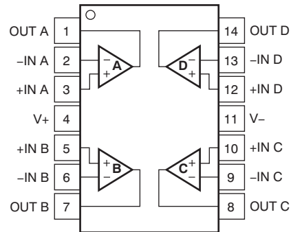
Pin Functions
