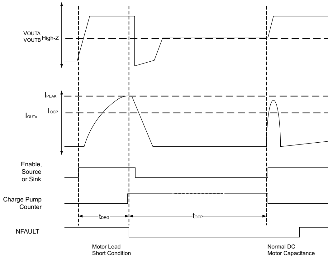
Figure 6. Overcurrent Control Timing
