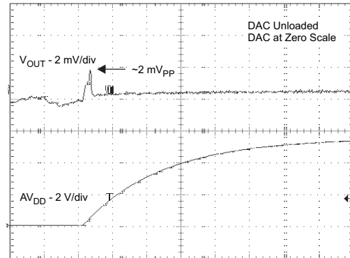
POWER-ON GLITCH RESET TO ZERO SCALE
