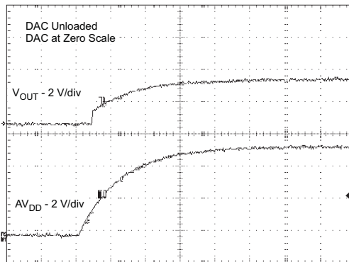
POWER-ON GLITCH RESET-TO-MID SCALE
