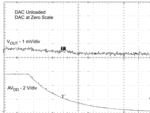
POWER-OFF GLITCH
