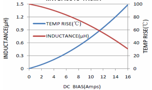
MWSA0518-1R5MT
