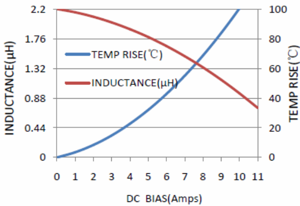
MWSA0518-2R2MT
