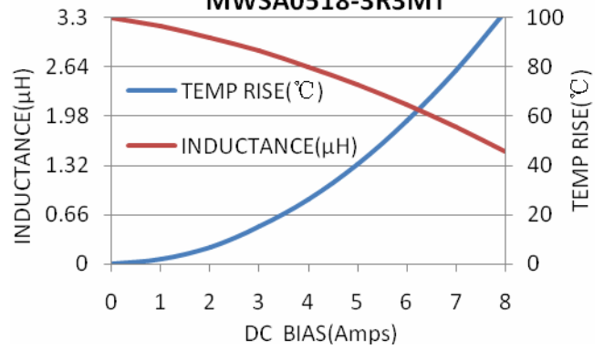
MWSA0518-3R3MT
