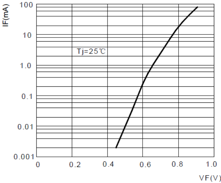
FIG5: Forward Current vs. Forward Voltage
