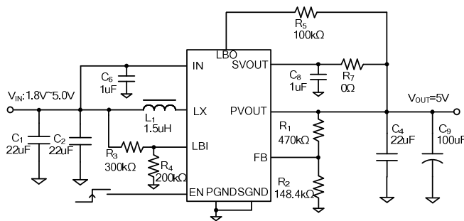
Figure 1. Schematic Diagram
