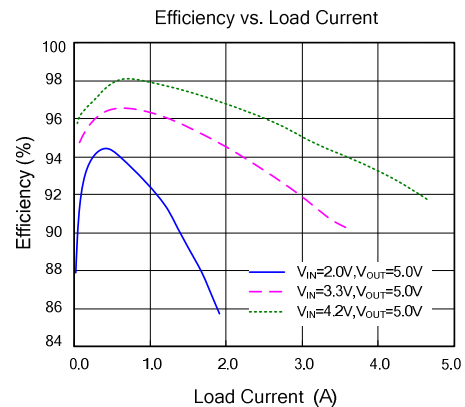
Figure 2. Efficiency Figure
