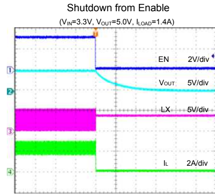
Time (400µs/div)
