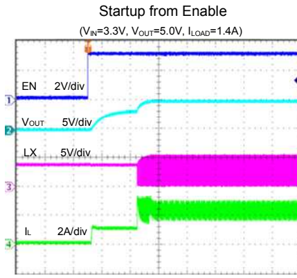
Time (1ms/div)
