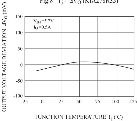
Fig.8 T_j - \Delta V_O (KIA278R35)
