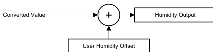
Figure 15. Humidity Offset
