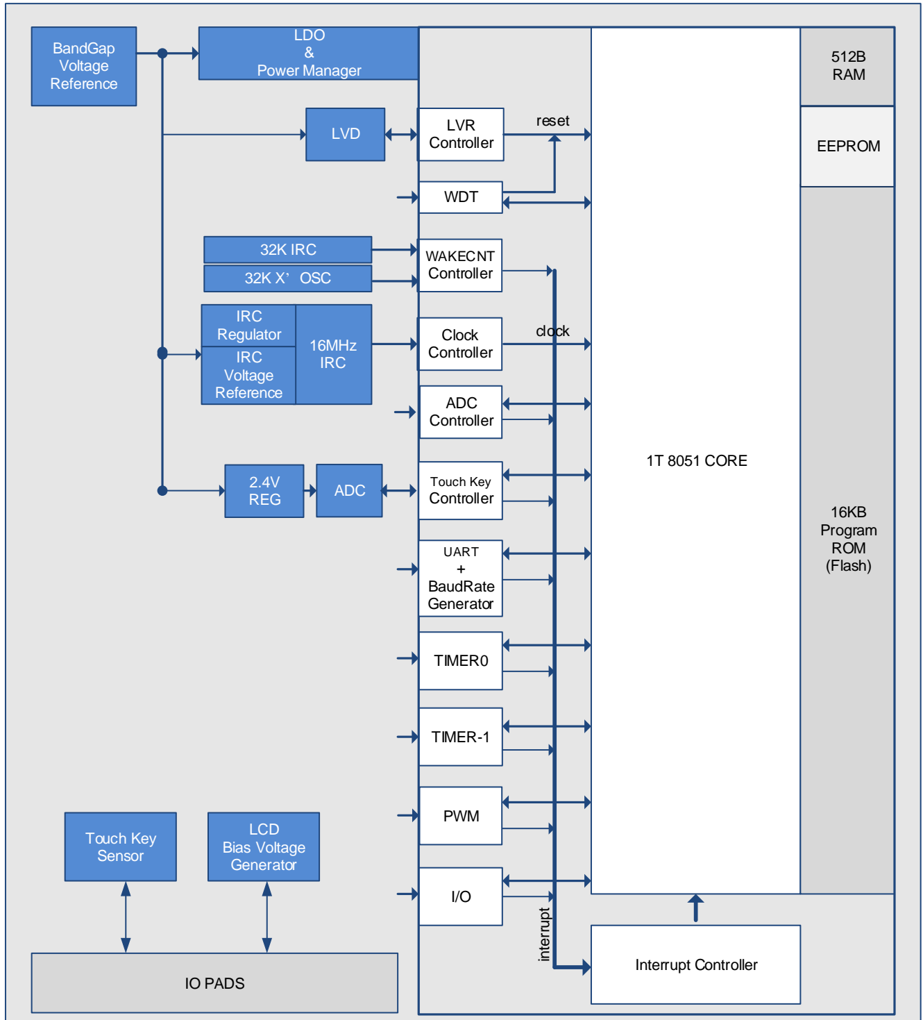
SC91F844 BLOCK DIAGRAM
