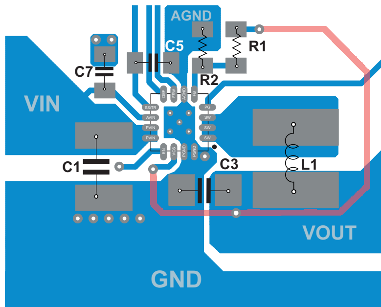
Figure 56. Layout Example
