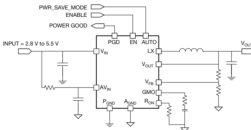
Fig. 1 - Typical Application Circuit for SiP12107
