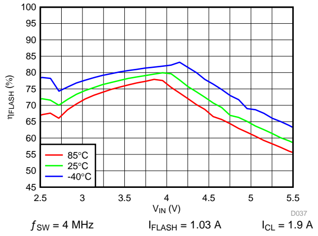
Figure 47. LED Flash Efficiency vs Input Voltage
