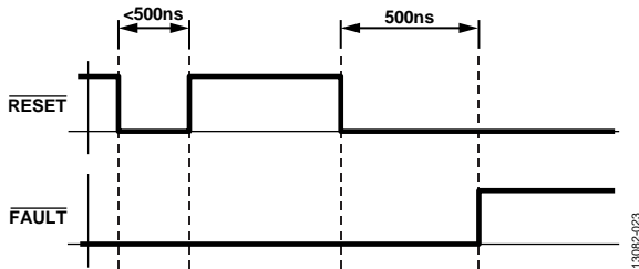
Figure 23. \overline{\text{RESET}} Timing
