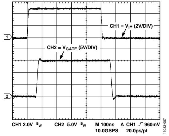
Figure 7. Typical Input to Output Waveform, 2 nF Load, 3.9 Ω Series Gate Resistor, V_{DD1} = 5 V , V_{DD2} = 15 V , V_{SS2} = 0 V
