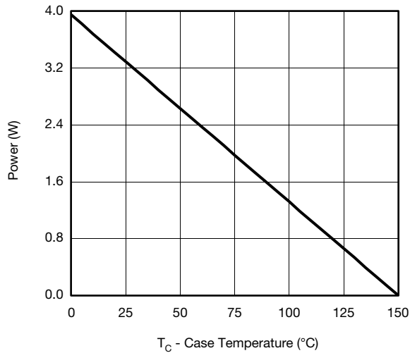
Power, Junction-to-Foot
