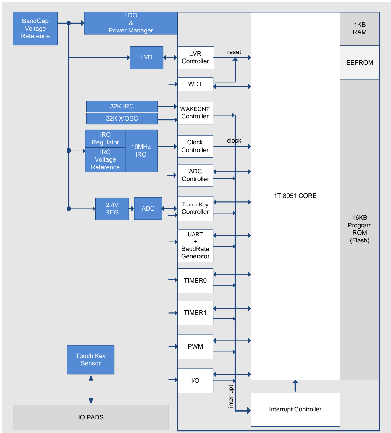
SC91F846 BLOCK DIAGRAM
