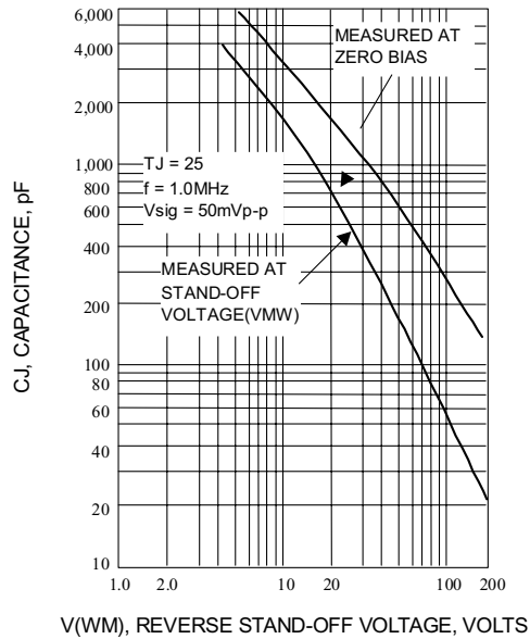
Fig. 4-TYPICAL JUNCTION CAPACITANCE
