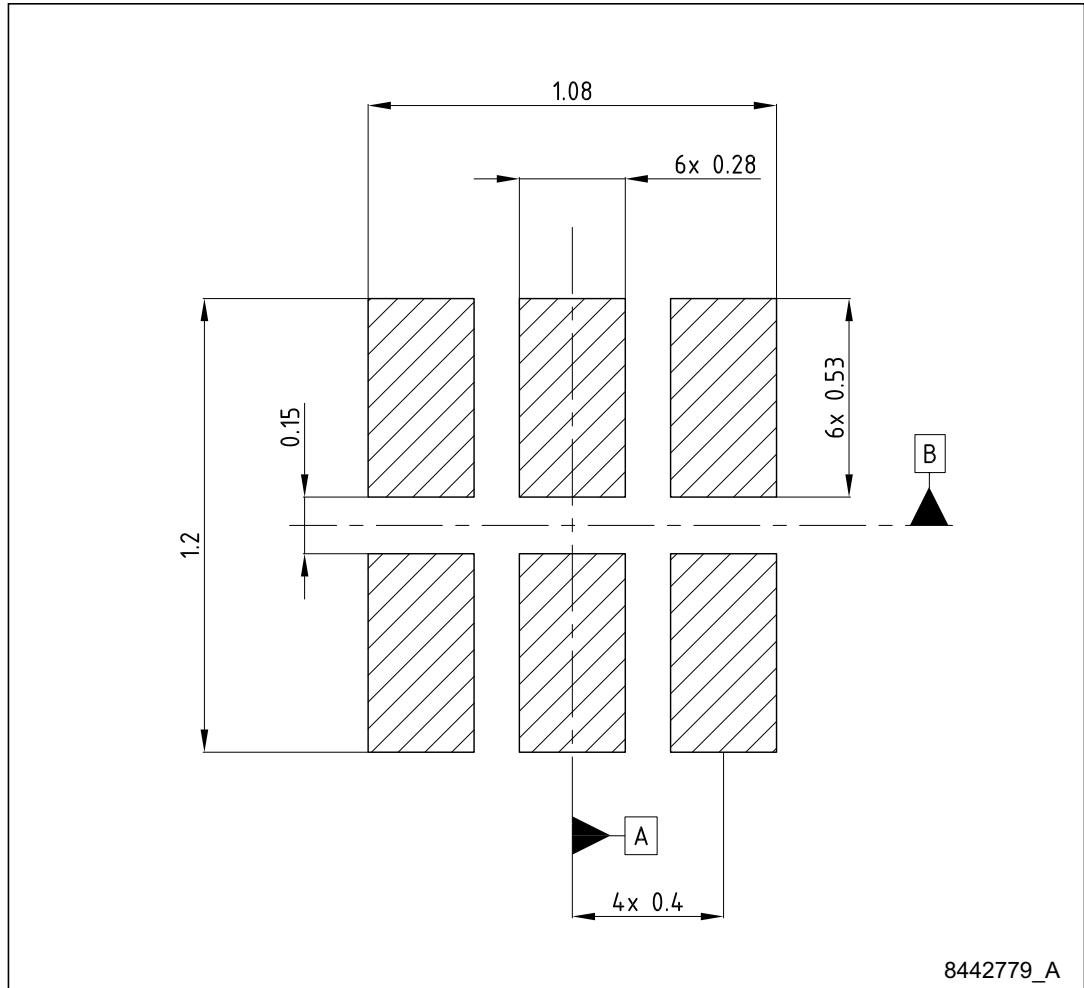
Figure 38. DFN6 1.2 x 1.3 footprint (dimensions in mm)
