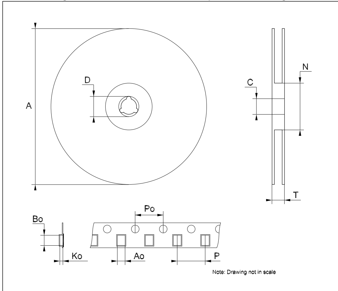
Figure 40. SOT23-5L and SOT323-5L tape and reel drawing
