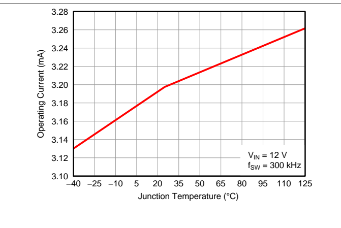
Figure 6. Operating Current vs Junction Temperature
