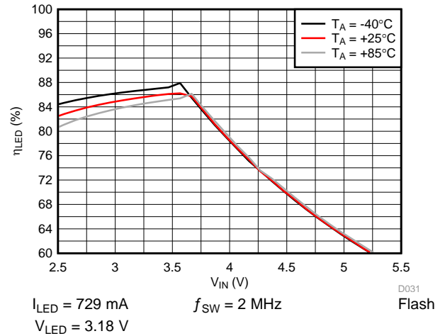
Figure 42. LED Efficiency vs Input Voltage
